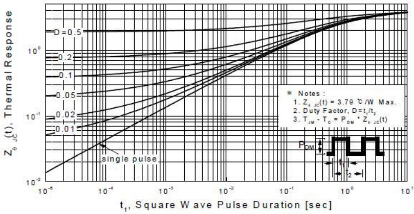
Figure 11-2. Transient Thermal Response Curve for TSP5N65M
