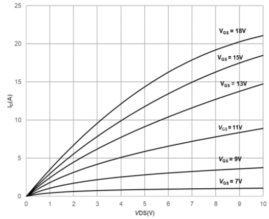
Fig2. Output Characteristics Tj=175°C
