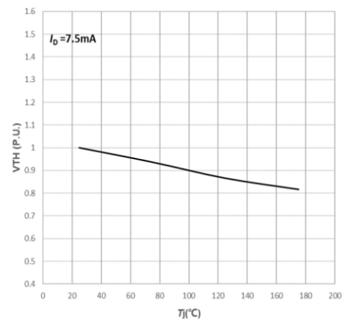
Fig6. Normalized Threshold Voltage vs. Temperature
