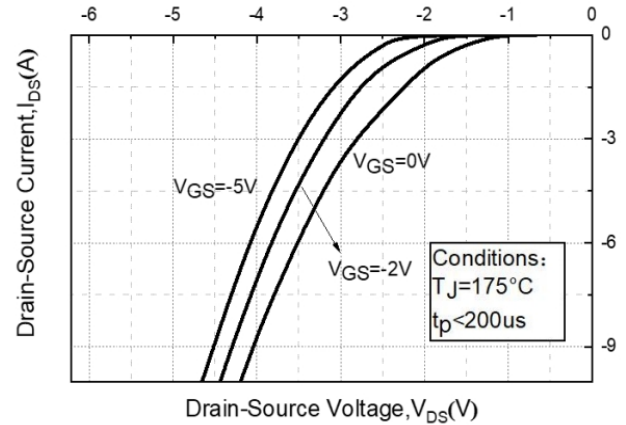
Fig10. Body Diode Characteristic at 175^\circ\text{C}
