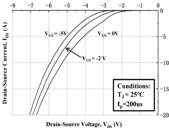
Fig9. Body Diode Characteristic at 25°C
