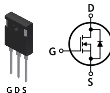
TO-247
