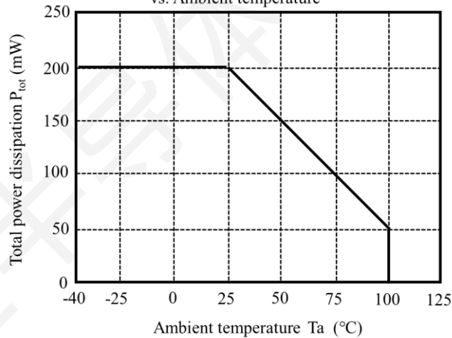
(Fig. 4) Total power dissipation vs. Ambient temperature
