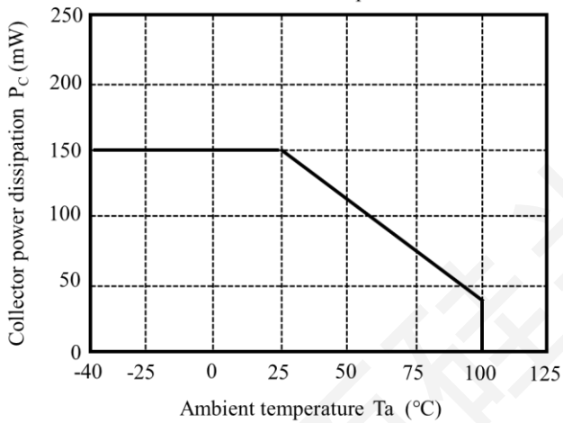
(Fig. 3) Collector power dissipation vs. Ambient temperature
