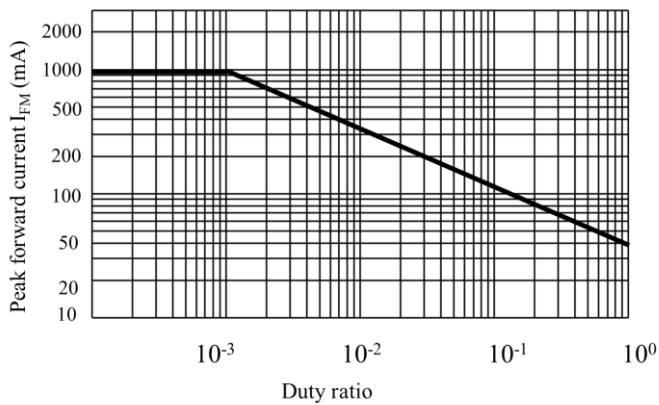
(Fig. 5) Peak forward current vs. Duty ratio Pulse width \leq 100 \mu s T_a = 25^\circ C
