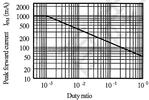
(Fig. 3) Peak forward current vs. duty ratio Pulse width \leq 100\mu\text{s} T_a = 25^\circ\text{C}
