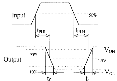
Timing chart
