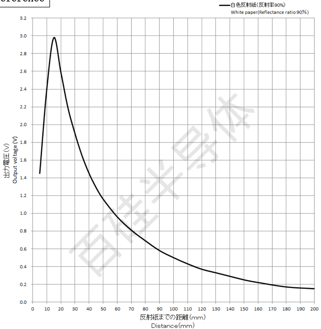
GP2Y0AF15XR 距離特性例 GP2Y0AF15XR Example of output distance characteristics
